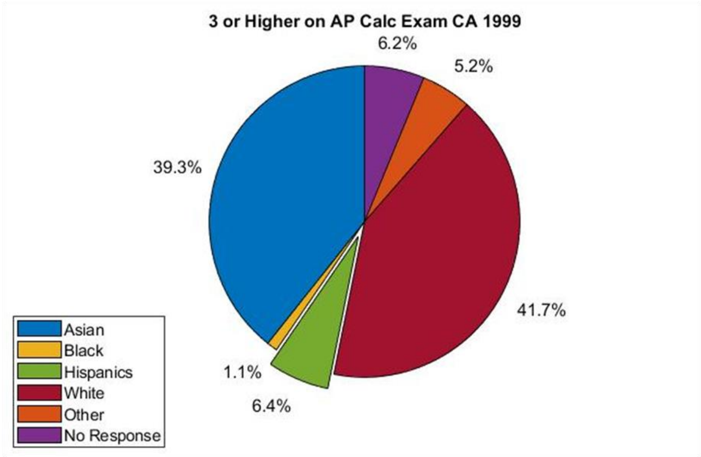
Figure 1. Distribution by race/ethnicity of California Test-Takers in 1999 who scored a 3 or higher on either AP calculus Exam. Source: College Board [9, 1999] and [17, 2019]
